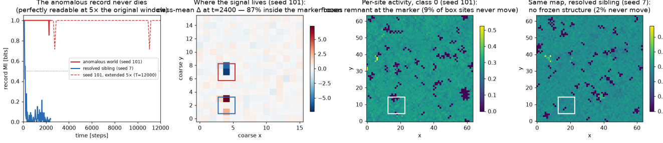
FIG. 3. The censored run, diagnosed: a spontaneously frozen record (scatter 0.42, one of five quenched worlds). Left: the anomalous world’s record never dies—it remains perfectly readable when the run is extended to 5\times the original window ( \approx 48 t_S )—while a resolved sibling world’s record dies on schedule. Middle-left: the class-mean coarse difference \Delta at t = 2400 — 87% inside the marker boxes remnant at the marker (9% of box sites never move). Right two panels: per-site activity maps; the anomalous world holds a frozen solid remnant of the marker (never-move sites with occupancy 0.93 in the own box, 0.07–0.15 in the opposite, initially empty box), absent in the sibling. A fully occupied or empty 2 \times 2 block is a fixed point of every rule, so a stalled erosion stores the record indefinitely: the \tau_{\text{mode}} \rightarrow \infty limit of Eq. (10), realized by quenched disorder.
