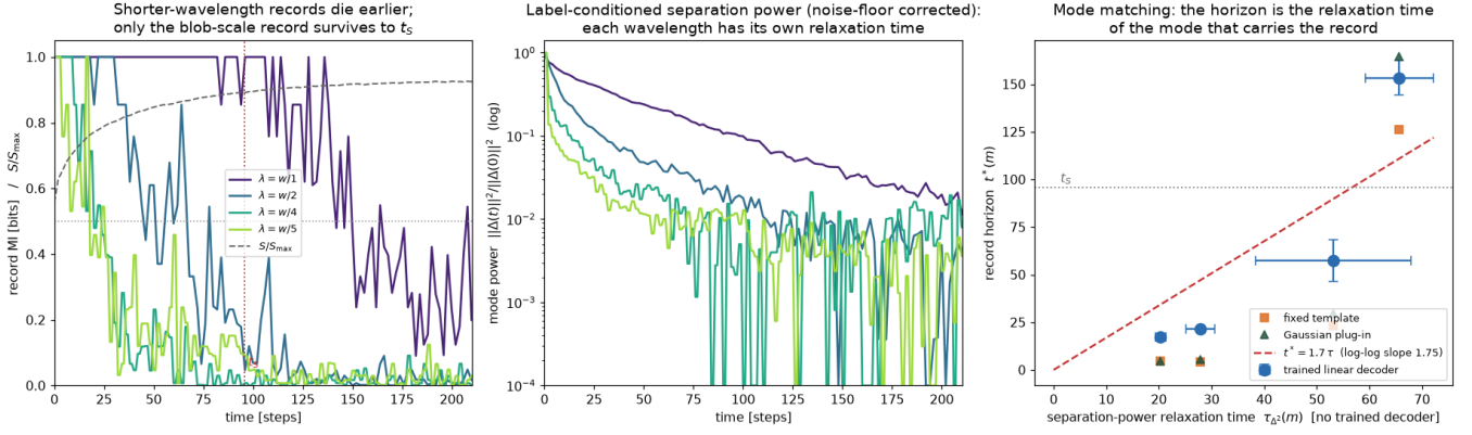
FIG. 5. The horizon is mode-matched (lattice gas, stripe-phase records at wavelengths \lambda = w/m , m = 1, 2, 4, 5 ; K = 40 , three seeds). Left: record MI for each wavelength, with S/S_{\max} (dashed) and t_S marked: shorter-wavelength records die earlier at fixed entropy clock ( t_S flat to 2.3%, t^* spanning 9\times ). Middle: label-conditioned separation power \|\Delta(t)\|^2 on a log scale—each wavelength has its own relaxation time. Right: t^*(m) against \tau_{\Delta^2}(m) with the three readouts; each mode’s lifetime is reconstructed by its own \tau_M \ln(A_M/\theta_M) to 1–5% (see text).
