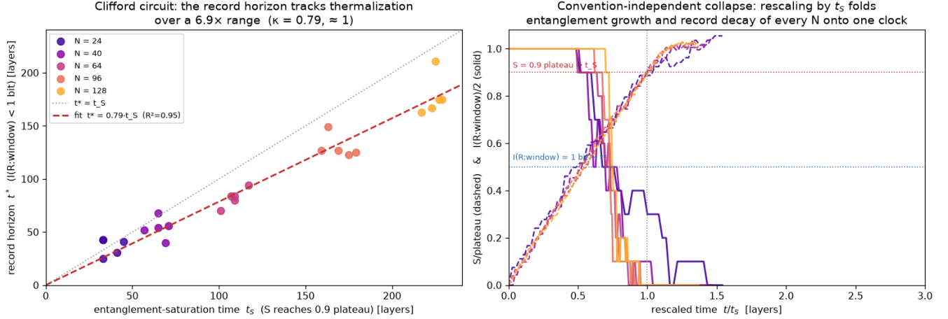
FIG. 6. Universality II: exactly reversible quantum (Clifford) circuits ( N = 24 –128 qubits, five circuit seeds per size). Left: record horizon vs. entanglement-saturation time; t^* = 0.79 t_S ( R^2 = 0.95 ) over a 6.9× range, per-size ratios flat. Right: t/t_S collapse of entanglement growth (dashed) and record decay (solid) for all sizes. A statevector control with Haar-random gates (see text) confirms the behaviour is not a stabilizer artifact.
