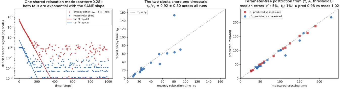
FIG. 3. One slow mode, two thresholds (lattice gas, 5 scrambling rates \times 3 seeds). Left: for one example condition, the entropy deficit S_{eq} - S(t) and the record signal I(F; \hat{F})(t) on a logarithmic scale; both tails are exponential with the same slope. Middle: fitted \tau_M against \tau_S for all runs; the ratio is 0.92 \pm 0.30 , flat over a 7.6\times range of absolute timescales. Right: reconstruction of both crossing times from the fitted (\tau, A) and the thresholds, Eq. (9): median error 5% ( t^* ) and 1% ( t_S ); leave-one-out prediction across seeds performs comparably (see text).
