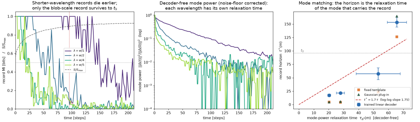
FIG. 4. The horizon is mode-matched (lattice gas, stripe-phase records at wavelengths \lambda = w/m , m = 1, 2, 4, 5 ; K = 40 , three seeds). Left: record MI for each wavelength, with S/S_{max} (dashed) and t_S marked: shorter-wavelength records die earlier at fixed entropy clock ( t_S flat to 2.3%, t^* spanning 9\times ). Middle: decoder-free mode power \|\Delta(t)\|^2 on a log scale—each wavelength has its own relaxation time. Right: t^*(m) against \tau_{\Delta^2}(m) with the three readouts; each mode's lifetime is reconstructed by its own \tau_M \ln(A_M/\theta_M) to 1–5% (see text).
