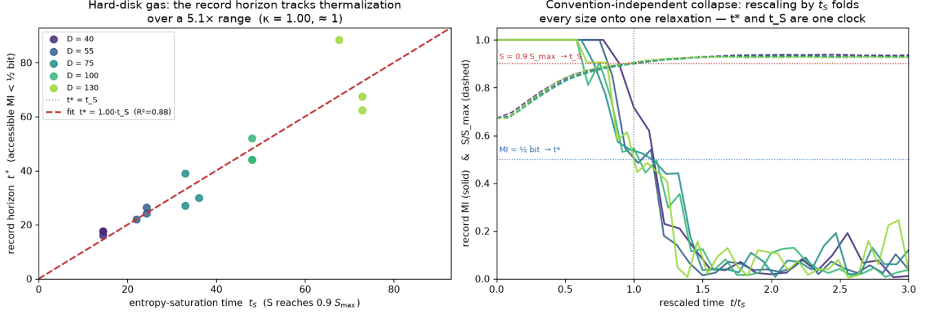
FIG. 5. Universality I: continuous hard-disk gas (self-similar size sweep, D = 40\text{--}130 , three seed-ensembles per size). Left: t^* vs. t_S ; t^* = 1.00 t_S over a 5.1\times range with flat per-size ratios. Right: rescaling time by t_S folds every size onto one relaxation — t^* and t_S are one clock
