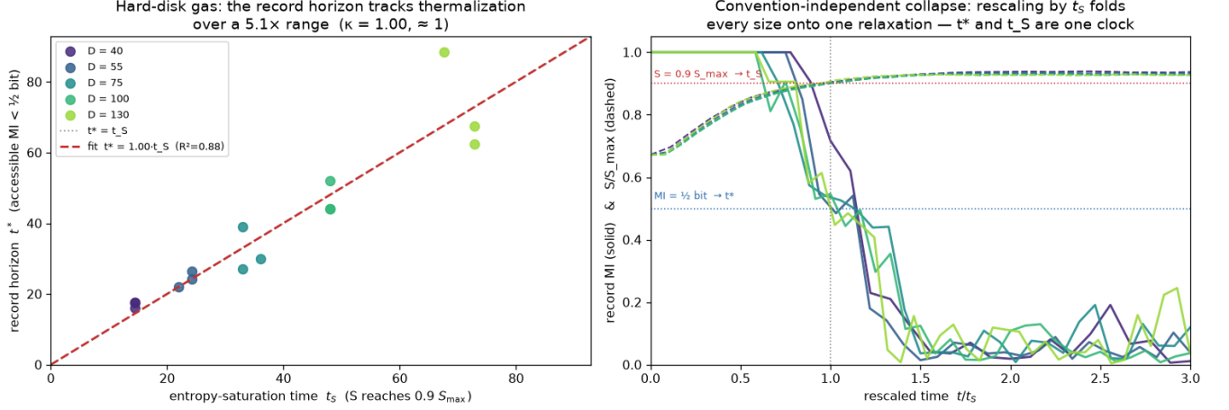
FIG. 6. Universality I: continuous hard-disk gas (self-similar size sweep, D = 40 – 130 , three seed-ensembles per size). Left: t^* vs. t_S ; t^* = 1.00 t_S over a 5.1\times range with flat per-size ratios. Right: rescaling time by t_S collapses the record MI (solid) and the entropy relaxation (dashed) of every size onto single master curves. The complementary mode-mismatch control is measured in Fig. 7.
