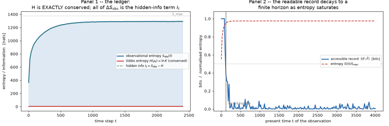
FIG. 1. Bookkeeping (bit-reversible lattice gas). Left ( K = 64 worlds, L = 128 , b = 8 ): the fine-grained entropy H of the evolving microstate ensemble is conserved to machine precision while the observational entropy S_{\text{obs}} rises; by the identity Eq. (4) the rise is the hidden-information term I . Right (parallel runs, K = 64 , L = 64 ): the accessible record I(F; \hat{F}) of a planted one-bit fact decays from 1.000 to 0.006 bit as the gas thermalizes.
