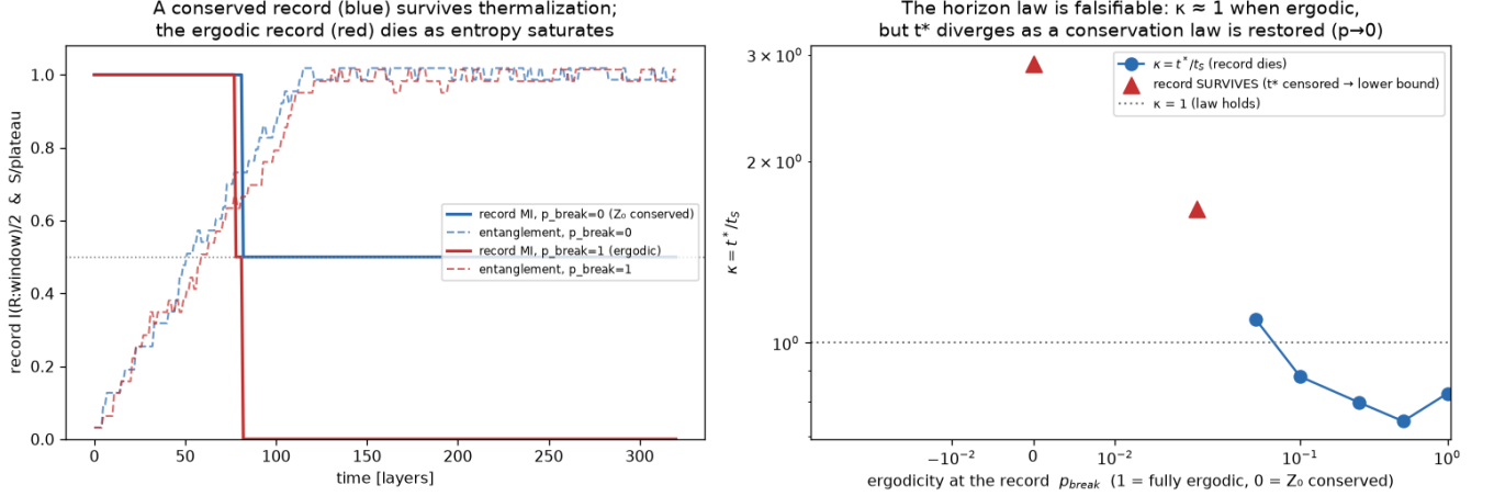
FIG. 9. The law fails where it must (Clifford chain, N = 64 ; a tunable Z_0 -conserving gate protects the record with probability 1 - p_{\text{break}} ). Left: example trajectories—under full scrambling the record dies as entanglement saturates, while the protected record survives arbitrarily long although the bulk thermalizes identically. Right: \kappa = t^*/t_S against p_{\text{break}} ; the ratio is order one in the ergodic regime and diverges (censored points are lower bounds) as the conservation law is restored, while t_S stays flat.
