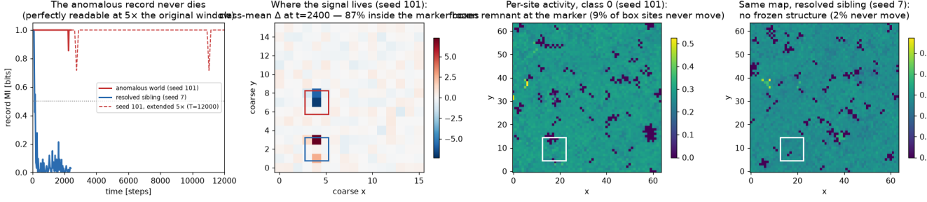
FIG. 3. The censored run, diagnosed: a spontaneously frozen record (scatter 0.42, one of five quenched worlds). Left: the anomalous world’s record never dies—it remains perfectly readable when the run is extended to 5\times the original window ( \approx 48 t_S )—while a resolved sibling world’s record dies on schedule. Middle-left: the class-mean coarse difference \Delta at t = 2400 — 87% inside the marker boxes remnant at the marker (9% of box sites never move). Right two panels: per-site activity maps; the anomalous world holds a frozen solid remnant of the marker (never-move sites with occupancy 0.93 in the own box, 0.07–0.15 in the opposite, initially empty box), absent in the sibling. A fully occupied or empty 2 \times 2 block is a fixed point of every rule, so a stalled erosion stores the record indefinitely: the \tau_{\text{mode}} \rightarrow \infty limit of Eq. (10), realized by quenched disorder.
