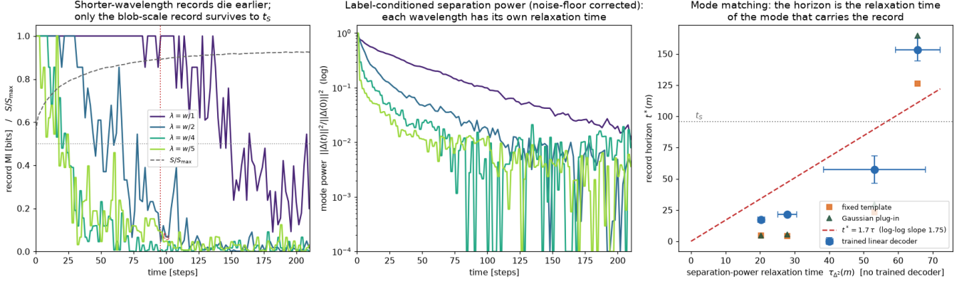
FIG. 5. The horizon is mode-matched (lattice gas, stripe-phase records at wavelengths \lambda = w/m , m = 1, 2, 4, 5 ; K = 40 , three seeds). Left: record MI for each wavelength, with S/S_{\max} (dashed) and t_S marked: shorter-wavelength records die earlier at fixed entropy clock ( t_S flat to 2.3%, t^* spanning 9\times ). Middle: label-conditioned separation power \|\Delta(t)\|^2 on a log scale—each wavelength has its own relaxation time. Right: t^*(m) against \tau_{\Delta^2}(m) with the three readouts; each mode’s lifetime is reconstructed by its own \tau_M \ln(A_M/\theta_M) to 1–5% (see text).
