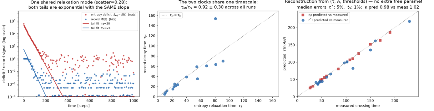
FIG. 4. One slow mode, two thresholds (lattice gas, 5 scrambling rates \times 3 seeds). Left: for one example condition, the entropy deficit S_{eq} - S(t) and the record signal I(F; \hat{F})(t) on a logarithmic scale; both tails are exponential with the same slope. Middle: fitted \tau_M against \tau_S for all runs; the ratio is 0.92 \pm 0.30 , flat over a 7.6\times range of absolute timescales. Right: reconstruction of both crossing times from the fitted (\tau, A) and the thresholds, Eq. (9): median error 5% ( t^* ) and 1% ( t_s ); leave-one-out prediction across seeds performs comparably (see text).
