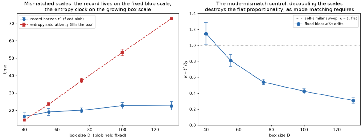
FIG. 7. The mode-mismatch control (hard-disk gas; blob and planted fact held at fixed absolute size while the box grows D = 40 – 130 ; three seed-ensembles per size). Left: the record horizon stays on the fixed blob scale ( t^* = 16.5 \rightarrow 22.5 ) while the entropy clock fills the growing box ( t_S = 14 \rightarrow 73 ). Right: \kappa = t^*/t_S drifts monotonically 1.15 \rightarrow 0.31 instead of staying flat; at D = 40 the fixed blob coincides with the self-similar one and \kappa matches Fig. 6. Decoupling the scales destroys the flat proportionality exactly as Eq. (10) requires.
