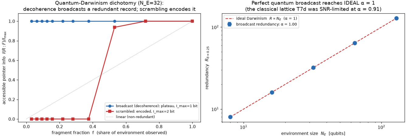
FIG. 11. Quantum Darwinism in the reversible circuit substrate . Left: partial-information profiles for a pointer bit broadcast into the environment (flat plateau: any small fragment carries the record) versus scrambled into it (step at half the environment: the record is encoded, not redundant). Right: effective redundancy of the broadcast record scales as R_\delta = N_E exactly ( \alpha = 1 , N_E = 8 –128)—the ideal limit the classical lattice approaches from below.
