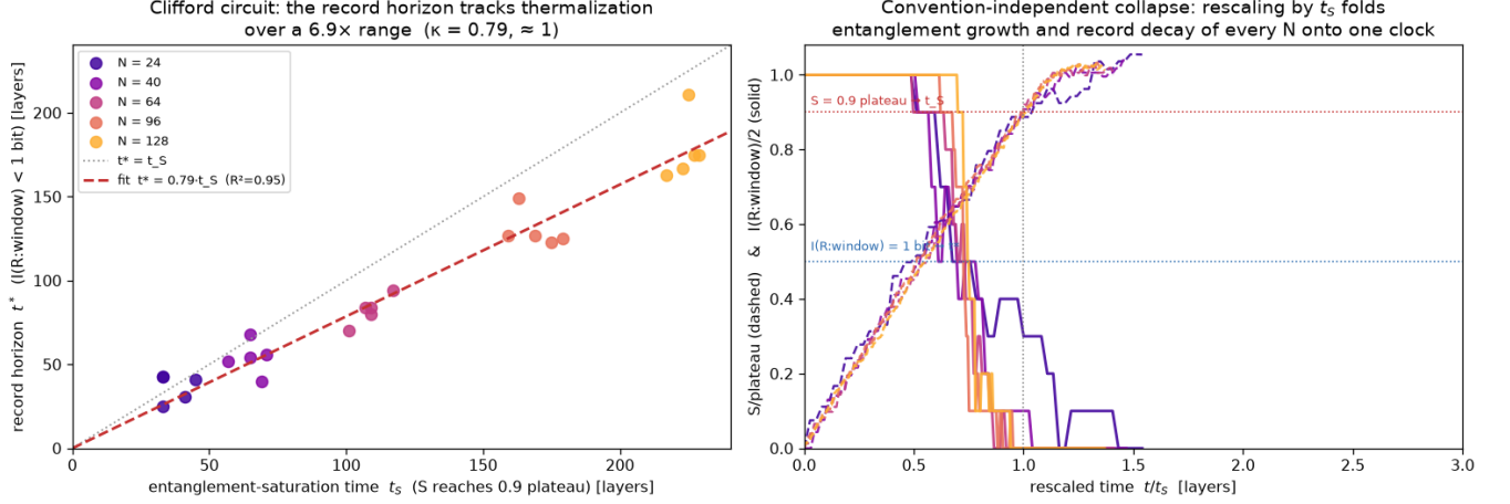
FIG. 8. Universality II: exactly reversible quantum (Clifford) circuits ( N = 24 – 128 qubits, five circuit seeds per size). Left: record horizon vs. entanglement-saturation time; t^* = 0.79 t_S ( R^2 = 0.95 ) over a 6.9\times range, per-size ratios flat. Right: t/t_S collapse of entanglement growth (dashed) and record decay (solid) for all sizes. A statevector control with Haar-random gates (see text) confirms the behaviour is not a stabilizer artifact.
