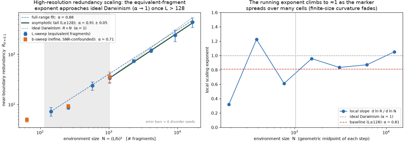
FIG. 10. Redundancy scaling toward ideal Darwinism (lattice gas, equivalent-fragment sweep L = 48 –512, i.e. N = (L/b)^2 up to 16,384; six disorder seeds). Left: near-boundary effective redundancy R_{\delta=0.1} vs. N ; the full-range exponent is 0.88, the L \geq 128 tail 0.91 \pm 0.05 (extrapolating to \alpha_\infty = 0.92 \pm 0.04 , conservatively; see text), while the SNR-confounded refinement sweep stays at \alpha = 0.71 . Right: the local slope d \ln R / d \ln N climbs to \approx 1 at the largest sizes as the small- L curvature fades.
