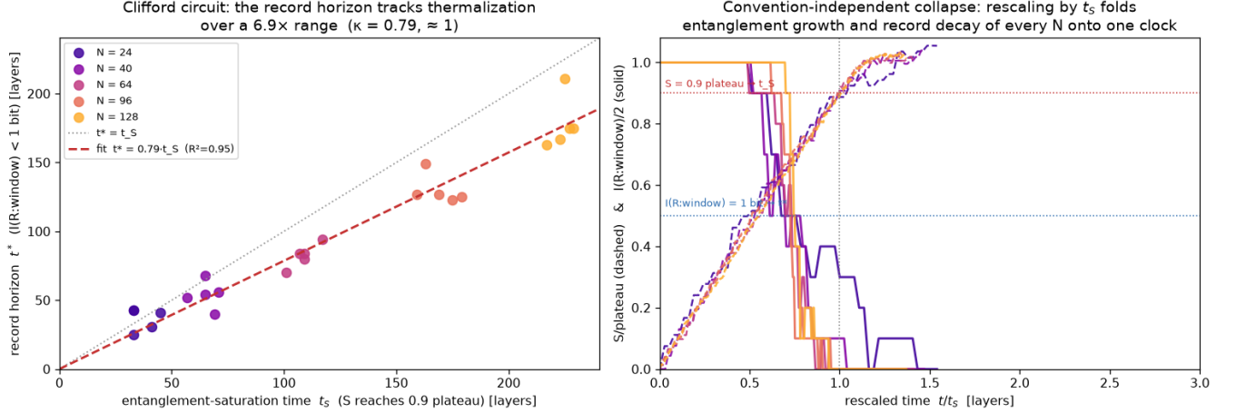
FIG. 8. Cross-substrate corroboration II: exactly reversible quantum (Clifford) circuits ( N = 24 –128 qubits, five circuit seeds per size). Left: record horizon vs. entanglement-saturation time; t^* = 0.79 t_S ( R^2 = 0.95 ) over a 6.9\times range, per-size ratios flat. Right: t/t_S collapse of entanglement growth (dashed) and record decay (solid) for all sizes. A statevector control with Haar-random gates (see text) confirms the behaviour is not a stabilizer artifact.
