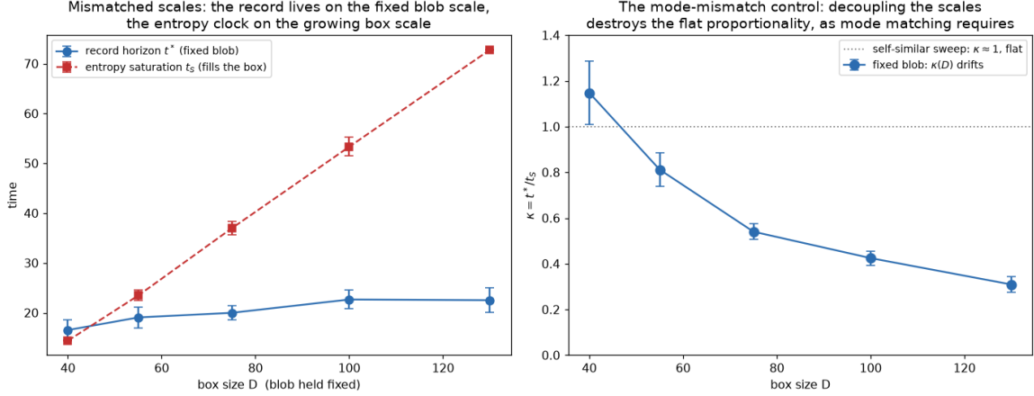
FIG. 7. The mode-mismatch control (hard-disk gas; blob and planted fact held at fixed absolute size while the box grows D = 40 –130; three seed-ensembles per size). Left: the record horizon stays on the fixed blob scale ( t^* = 16.5 \rightarrow 22.5 ) while the entropy clock fills the growing box ( t_S = 14 \rightarrow 73 ). Right: \kappa = t^*/t_S drifts monotonically 1.15 \rightarrow 0.31 instead of staying flat; at D = 40 the fixed blob coincides with the self-similar one and \kappa matches Fig. 6. Decoupling the scales destroys the flat proportionality exactly as Eq. (10) requires.
