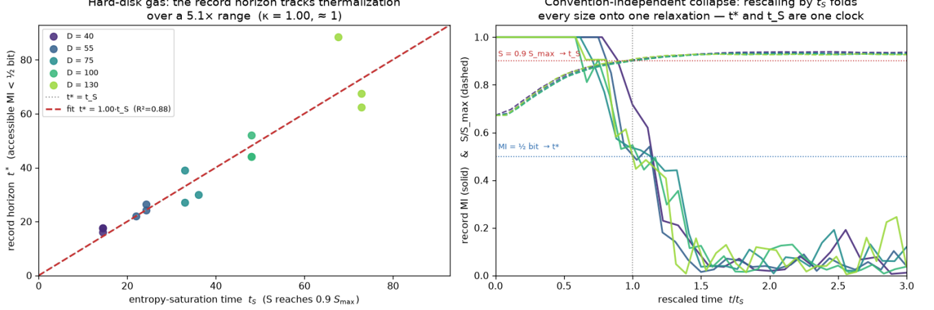
FIG. 6. Cross-substrate corroboration I: continuous hard-disk gas (self-similar size sweep, D = 40 –130, three seed-ensembles per size). Left: t^* vs. t_S ; t^* = 1.00 t_S over a 5.1 \times range with flat per-size ratios. Right: rescaling time by t_S collapses the record MI (solid) and the entropy relaxation (dashed) of every size onto single master curves. The complementary mode-mismatch control is measured in Fig. 7.
