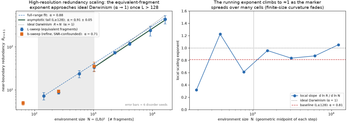
FIG. 10. Redundancy scaling toward ideal Darwinism (lattice gas, equivalent-fragment sweep L = 48 – 512 , i.e. N = (L/b)^2 up to 16,384 ; six disorder seeds). Left: near-boundary effective redundancy R_{\delta=0.1} vs. N ; the full-range exponent is 0.88 , the L \geq 128 tail 0.91 \pm 0.05 (extrapolating to \alpha_\infty = 0.92 \pm 0.04 , conservatively; see text), while the SNR-confounded refinement sweep stays at \alpha = 0.71 . Right: the local slope d \ln R / d \ln N climbs to \approx 1 at the largest sizes as the small- L curvature fades.
