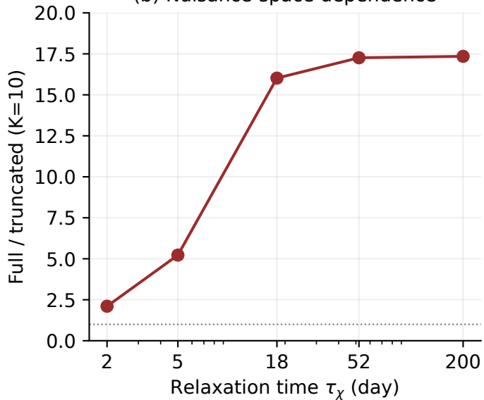
(b) Nuisance-space dependence
