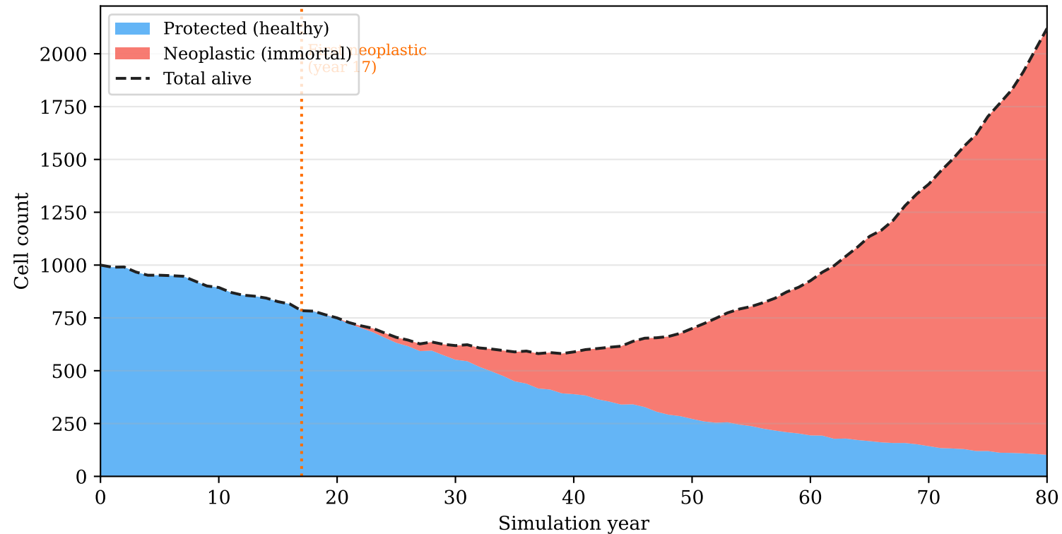
Figure 3 — Scenario 09 (Realistic Balanced): 80-year Cell Population Dynamics
