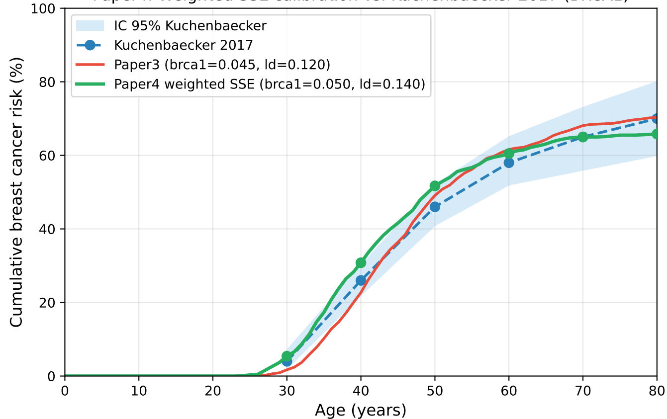
Paper4: Weighted SSE calibration vs. Kuchenbaecker 2017 (BRCA1)
