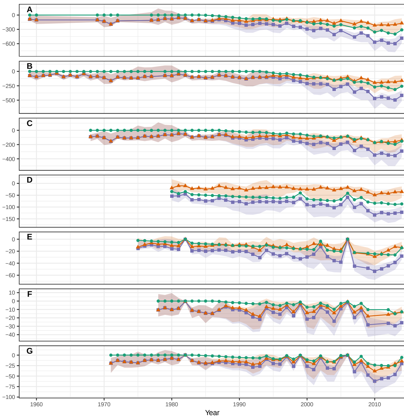
Climate Change Induced Shift in Streamflow (mm)
