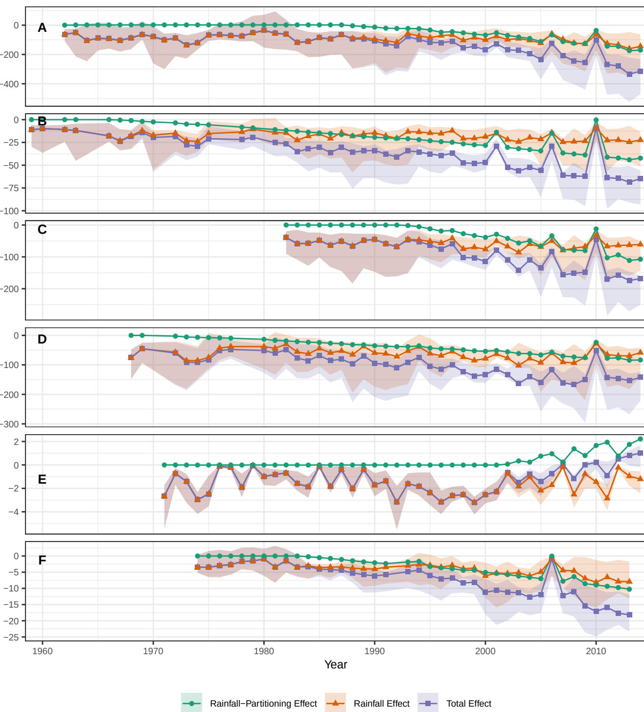
Climate Change Induced Shift in Streamflow (mm)
