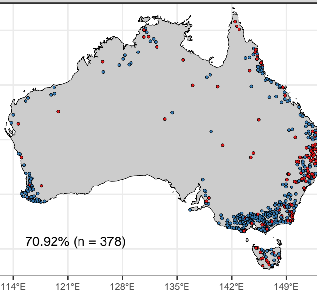
Rainfall Seasonality
