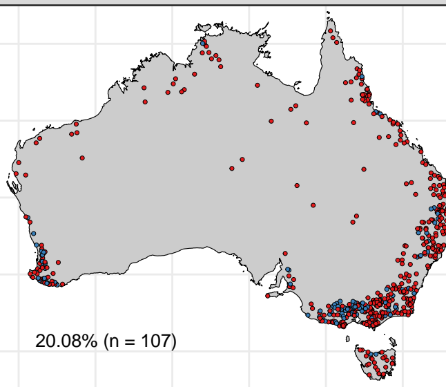
Rainfall Seasonality
