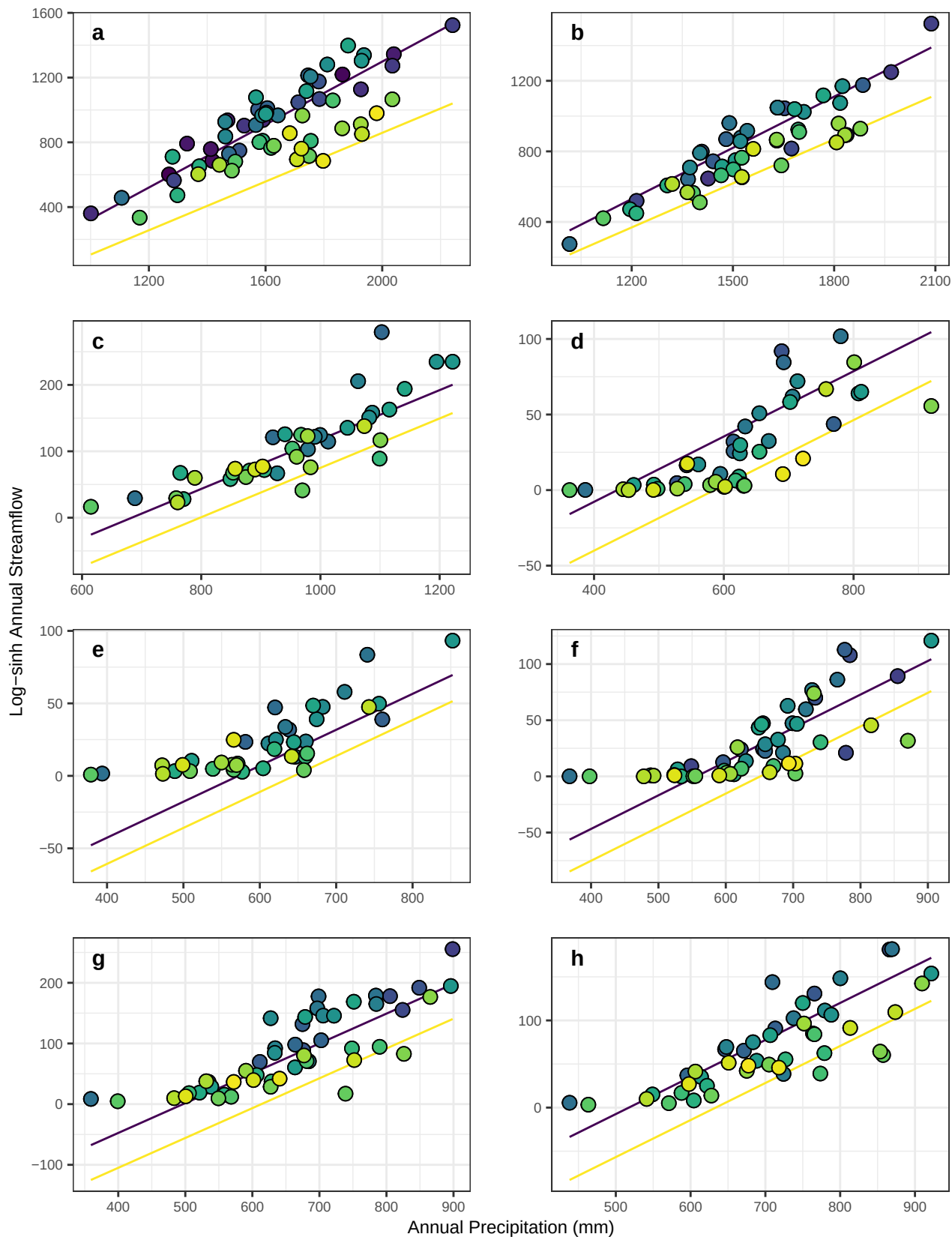
Modelled Rainfall-Runoff Relationship
