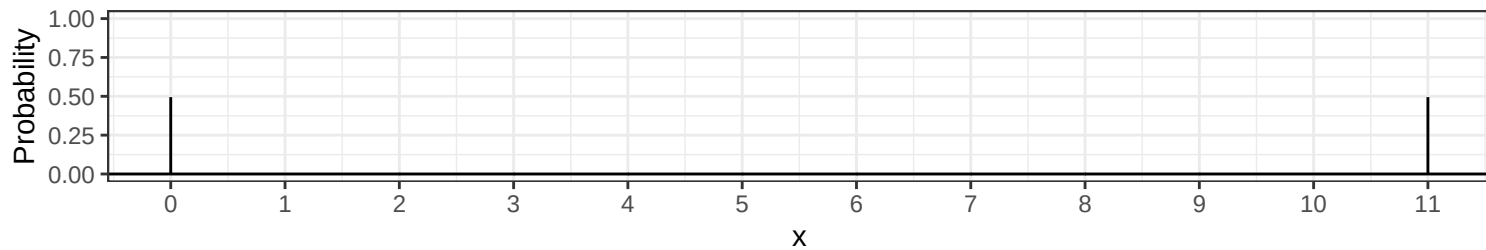
Distribution when \theta=1
