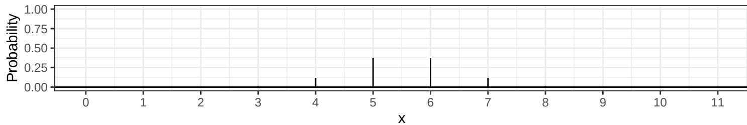
Distribution when \theta=1.5
