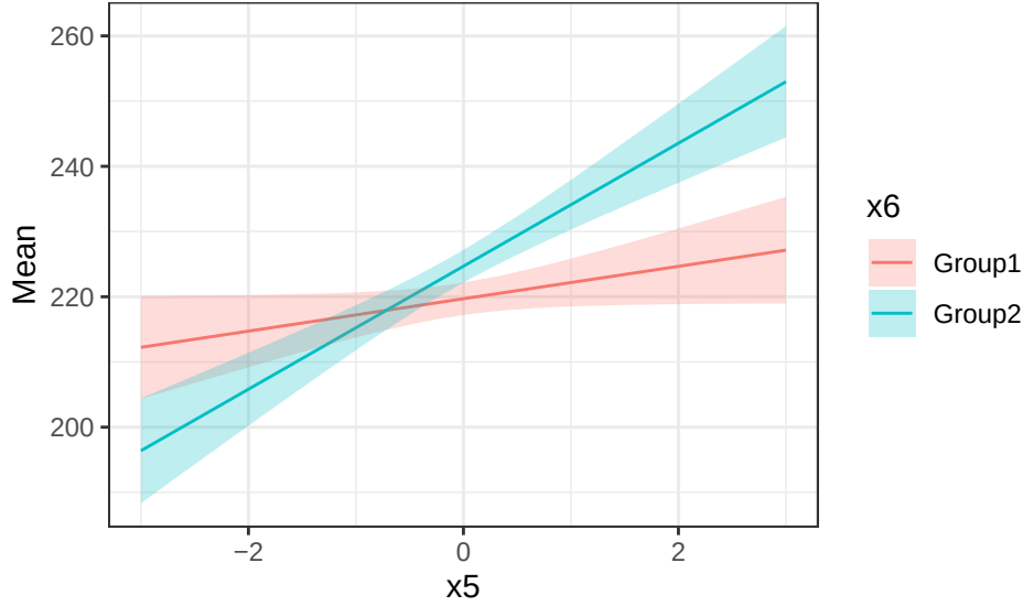
Figure 4: Estimated marginal trends for the model in Question 1.
