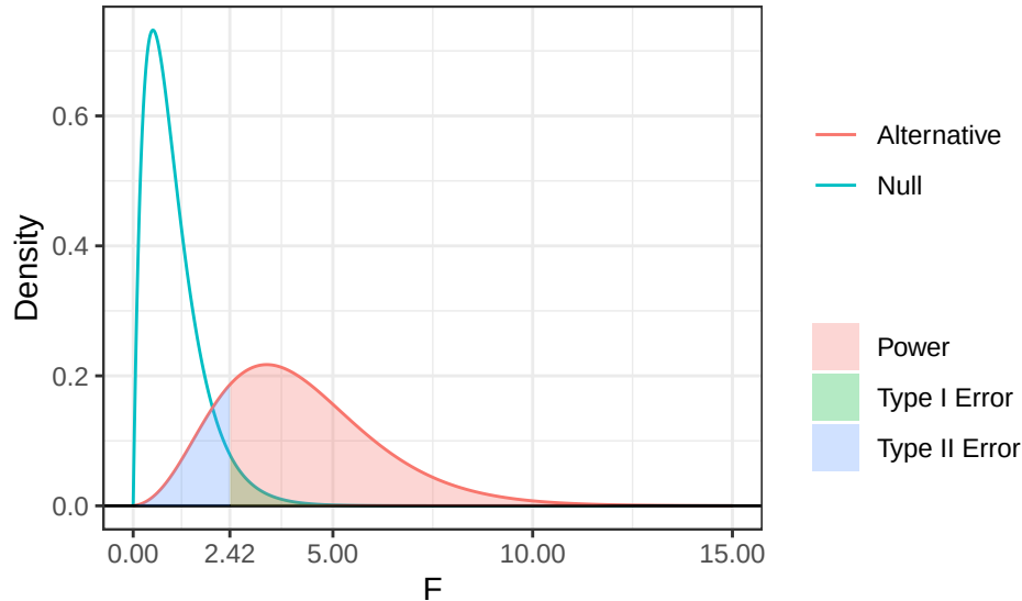
Figure 1: ( f = 0.25 , k = 5 ); n per group = 40 ( N = 200 )
