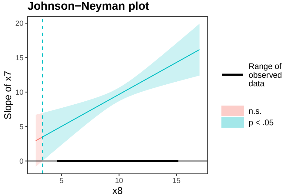
Figure 5: Johnson Neyman interval for the model in Question 1.
