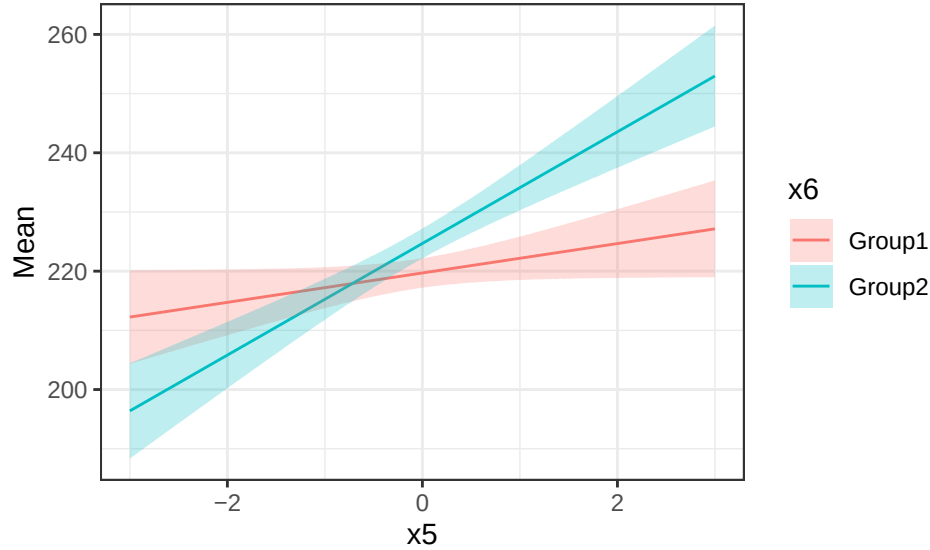
Figure 4: Estimated marginal trends for the model in Question 1.
