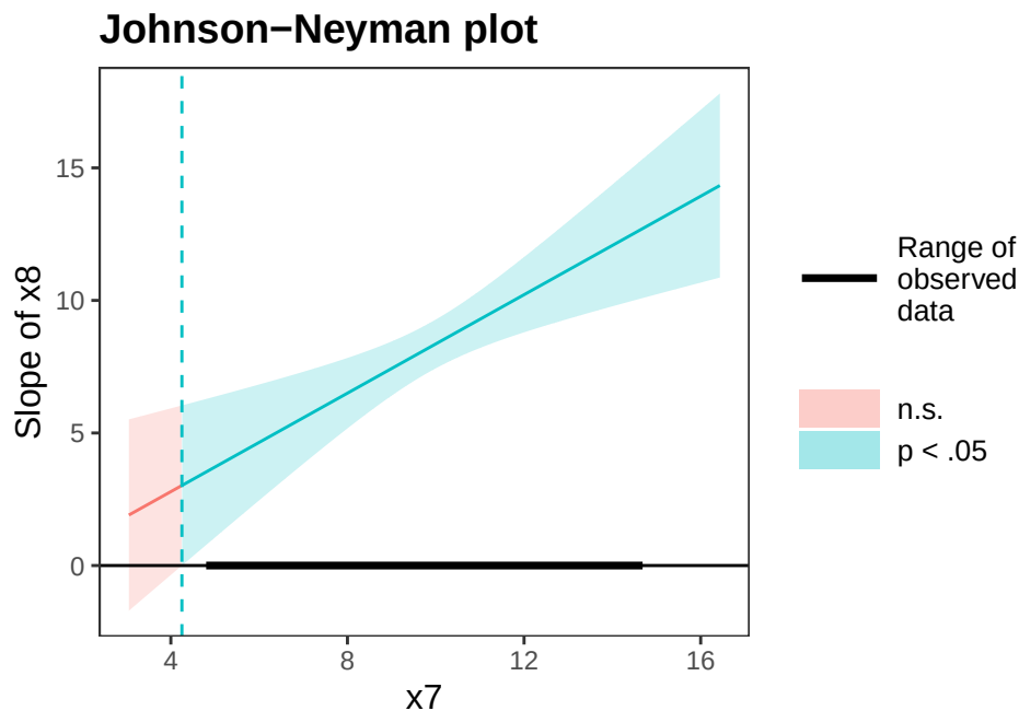
Figure 6: Johnson Neyman interval for the model in Question 1.
