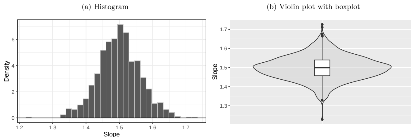
Figure 13: Distribution of the slope estimates
