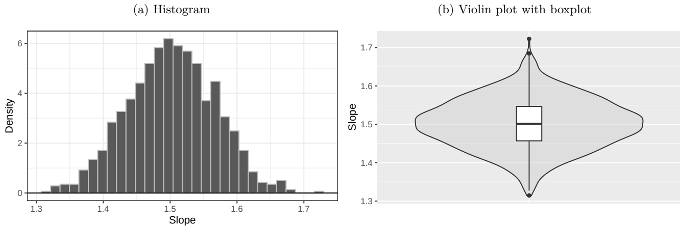
Figure 11: Distribution of the slope estimates
