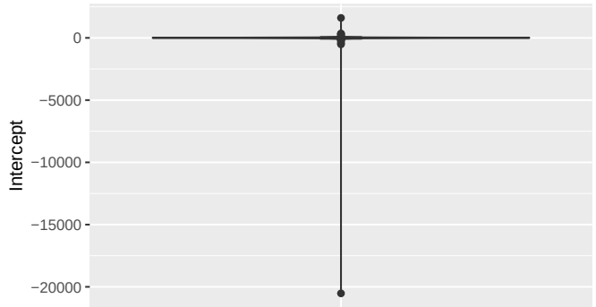
(b) Violin plot with boxplot
