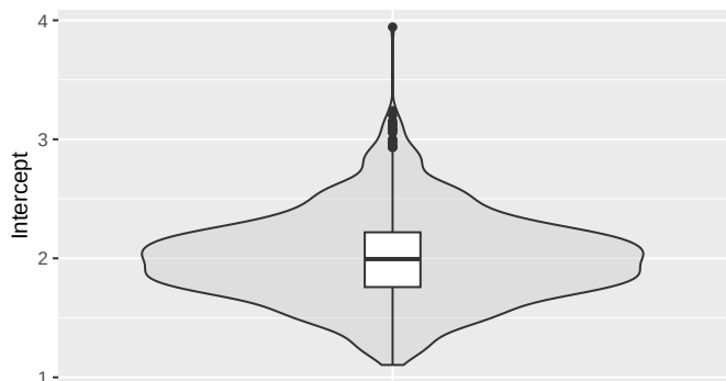
(b) Violin plot with boxplot
