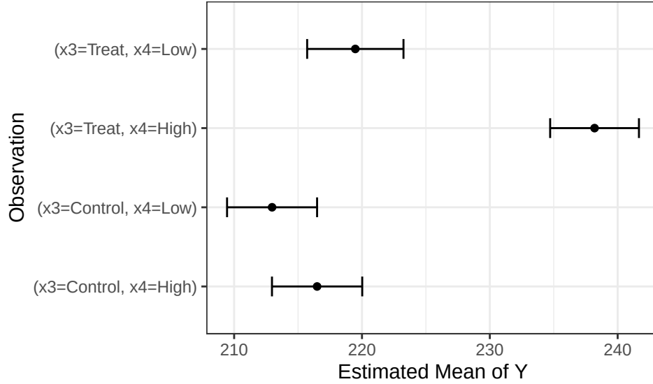
Figure 3: Estimated marginal means for the model in Question 1.
