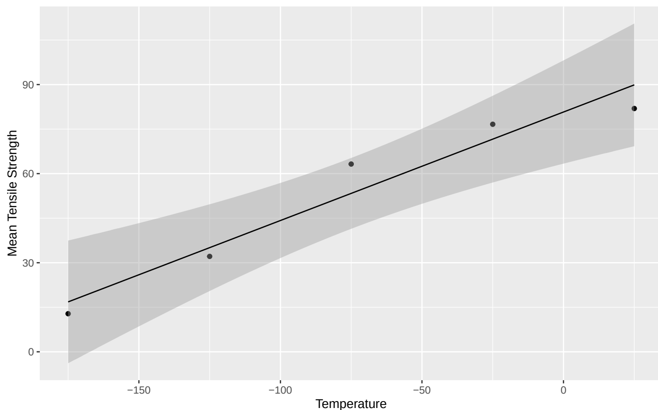
Figure 7: Regression on Conditional Means of Y
