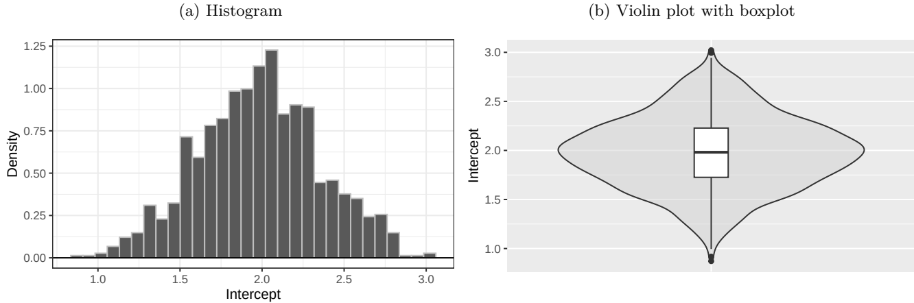
Figure 10: Distribution of the intercept estimates
