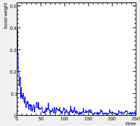
Boost weights vs tree
