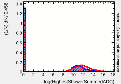
Input variable: log(HighestShowerSummedADC)
