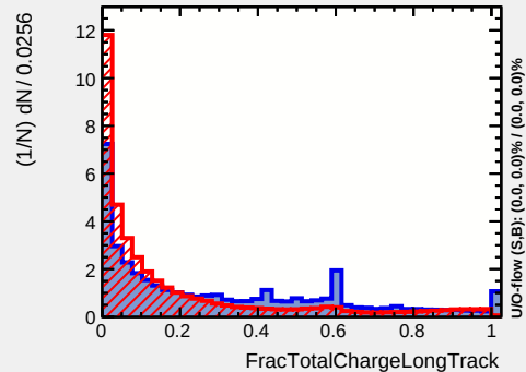
Input variable: FracTotalChargeLongTrack
