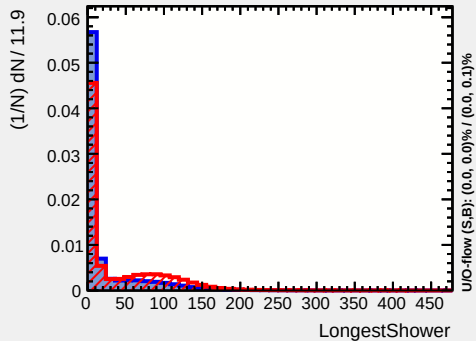
Input variable: LongestShower
