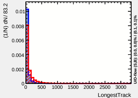
Input variable: LongestTrack
