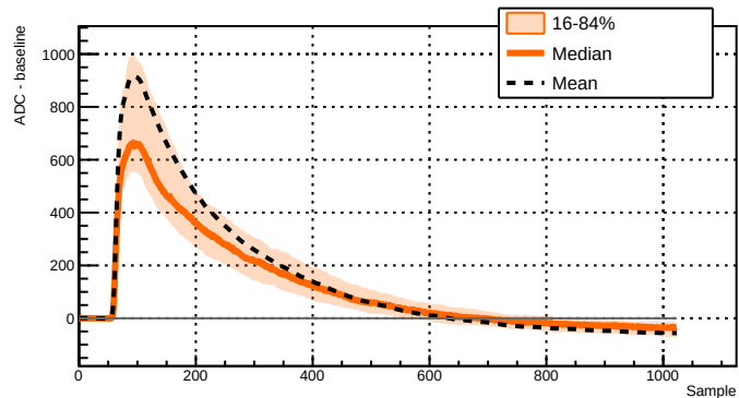
Run 043440 - Channel 2051 - 435 waveforms
