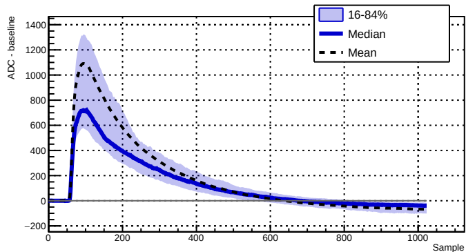
Run 043440 - Channel 2050 - 497 waveforms
