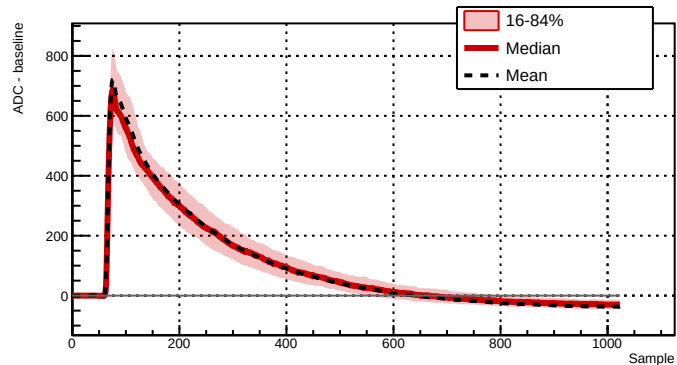
Run 043440 - Channel 2061 - 746 waveforms
