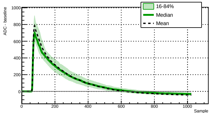
Run 043440 - Channel 2060 - 812 waveforms
