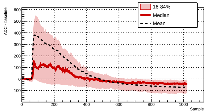
Run 043717 - Channel 2061 - 80 waveforms
