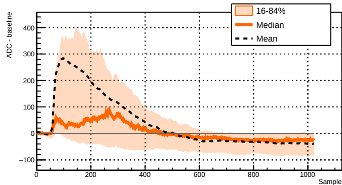
Run 043717 - Channel 2051 - 90 waveforms
