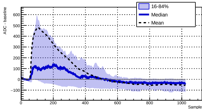
Run 043717 - Channel 2050 - 69 waveforms
