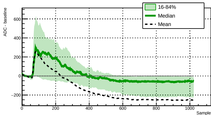
Run 043717 - Channel 2060 - 72 waveforms
