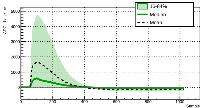
Run 043903 - Channel 2060 - 500 waveforms
