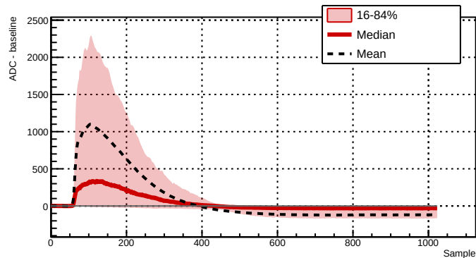
Run 043903 - Channel 2061 - 442 waveforms
