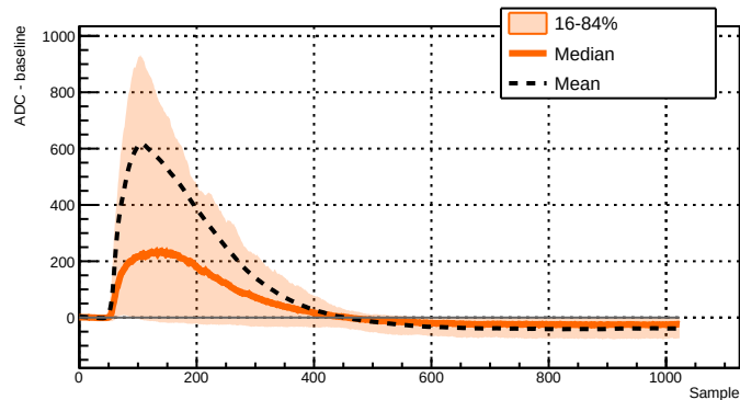
Run 043903 - Channel 2051 - 432 waveforms
