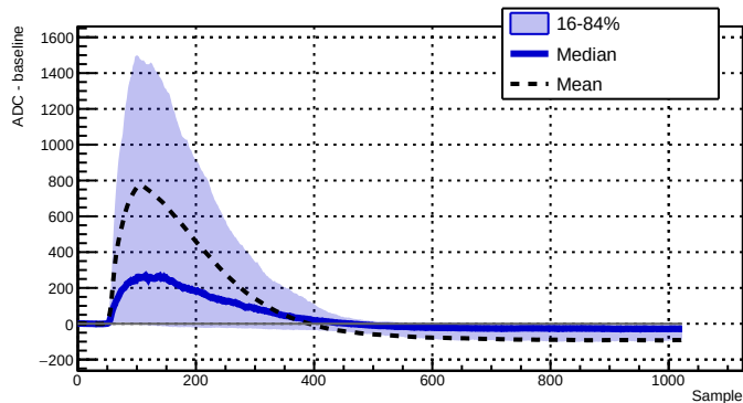
Run 043903 - Channel 2050 - 451 waveforms
