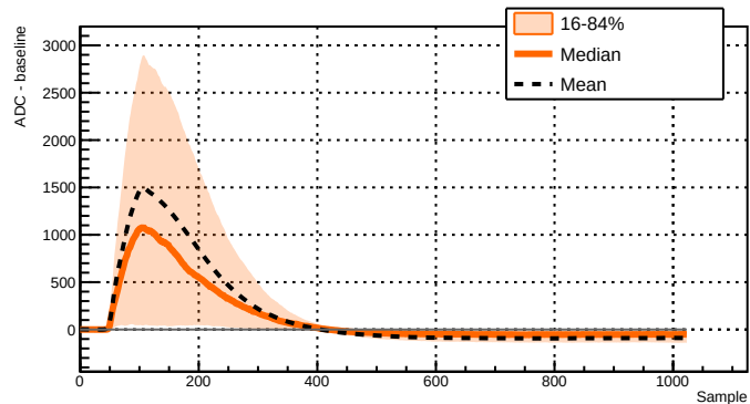
Run 044010 - Channel 2051 - 428 waveforms
