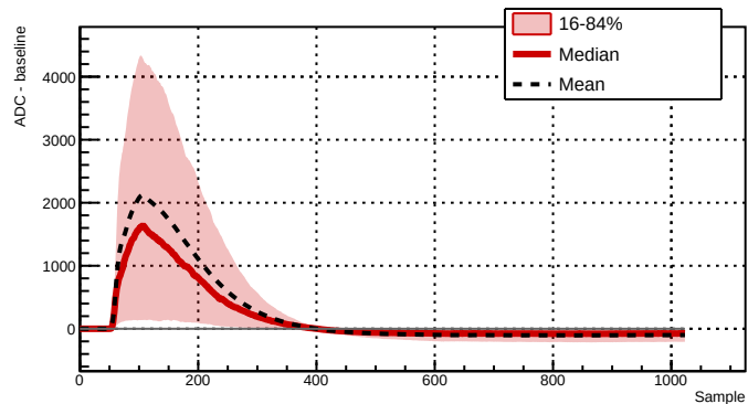
Run 044010 - Channel 2061 - 546 waveforms
