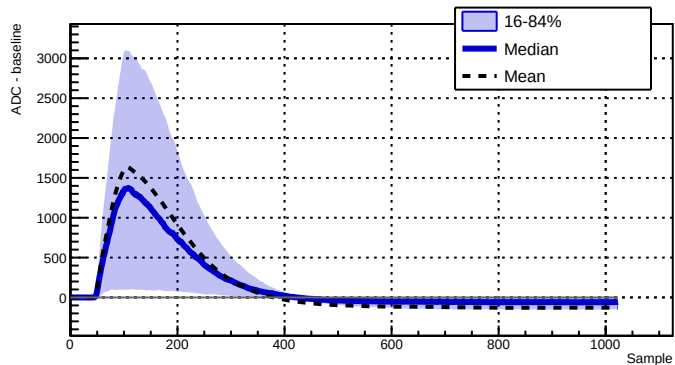
Run 044010 - Channel 2050 - 409 waveforms
