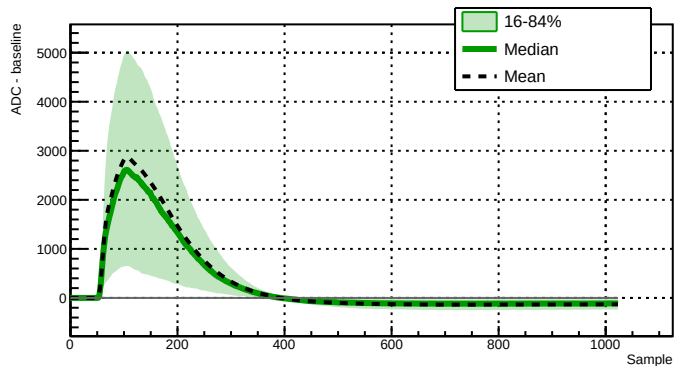
Run 044010 - Channel 2060 - 874 waveforms
