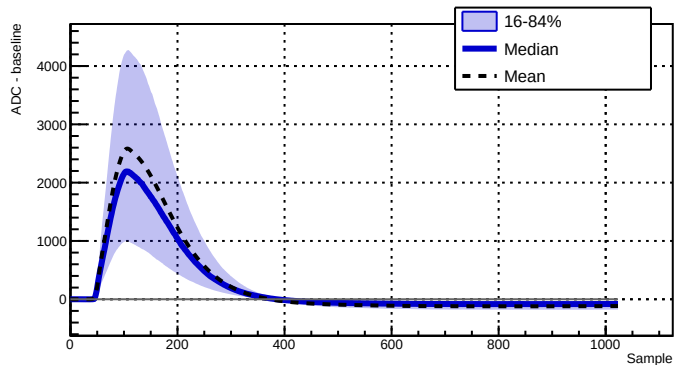
Run 044108 - Channel 2050 - 2612 waveforms
