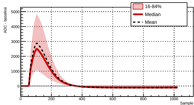
Run 044108 - Channel 2061 - 5179 waveforms
