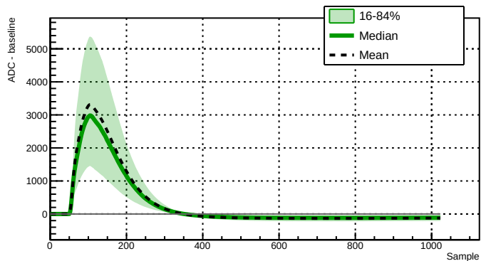
Run 044108 - Channel 2060 - 7251 waveforms
