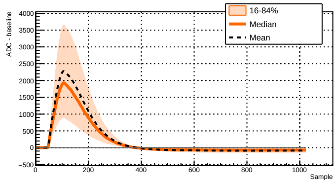
Run 044108 - Channel 2051 - 2927 waveforms
