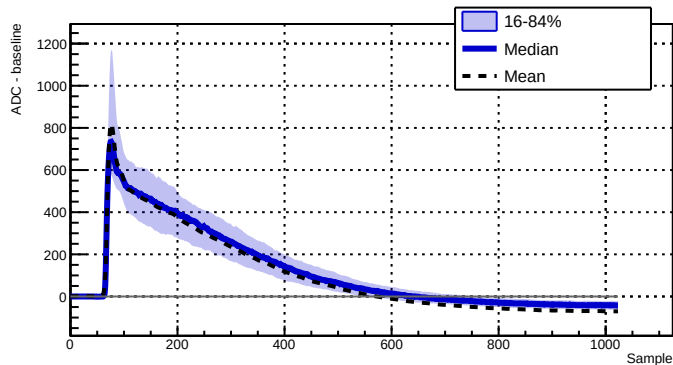
Run 043552 - Channel 2070 - 753 waveforms
