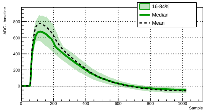
Run 043552 - Channel 2080 - 1436 waveforms
