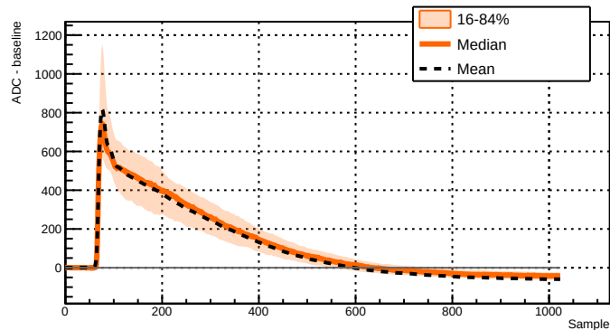
Run 043552 - Channel 2071 - 713 waveforms
