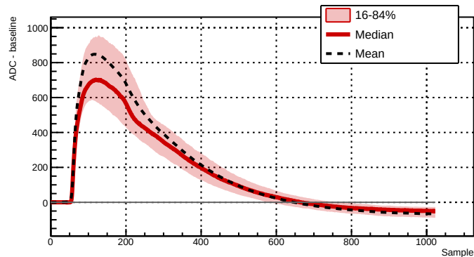
Run 043552 - Channel 2081 - 1663 waveforms
