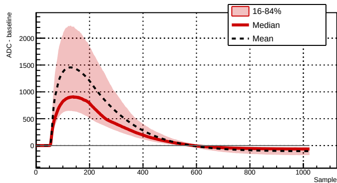
Run 043717 - Channel 2081 - 3075 waveforms
