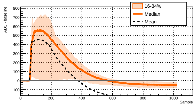
Run 043717 - Channel 2071 - 591 waveforms
