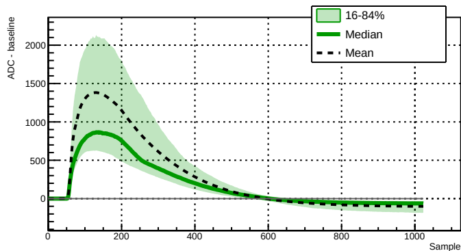
Run 043717 - Channel 2080 - 2496 waveforms
