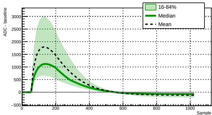
Run 043790 - Channel 2080 - 10428 waveforms
