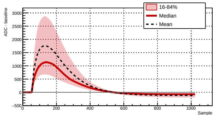
Run 043790 - Channel 2081 - 11544 waveforms
