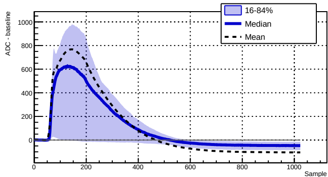
Run 043790 - Channel 2070 - 2897 waveforms
