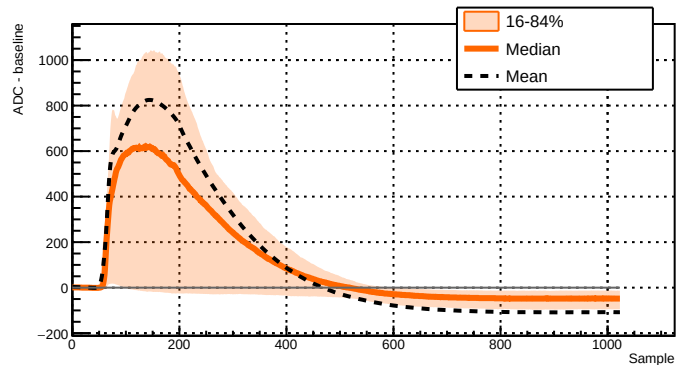
Run 043790 - Channel 2071 - 2964 waveforms
