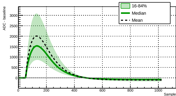
Run 043903 - Channel 2080 - 23897 waveforms
