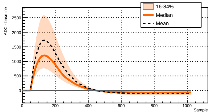
Run 043903 - Channel 2071 - 13402 waveforms
