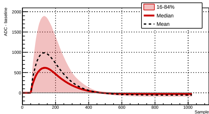
Run 043903 - Channel 2081 - 21078 waveforms
