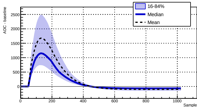
Run 043903 - Channel 2070 - 12670 waveforms
