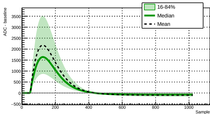
Run 044010 - Channel 2080 - 44017 waveforms
