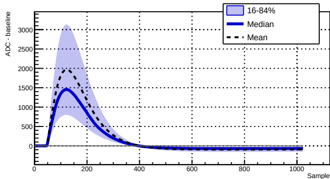
Run 044010 - Channel 2070 - 36482 waveforms
