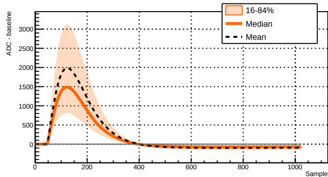
Run 044010 - Channel 2071 - 37218 waveforms
