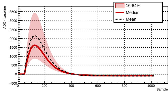
Run 044010 - Channel 2081 - 43721 waveforms
