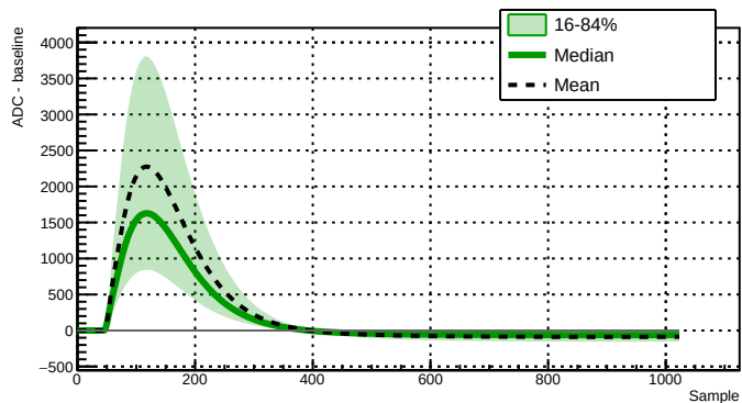
Run 044108 - Channel 2080 - 64584 waveforms
