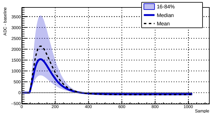
Run 044108 - Channel 2070 - 64741 waveforms
