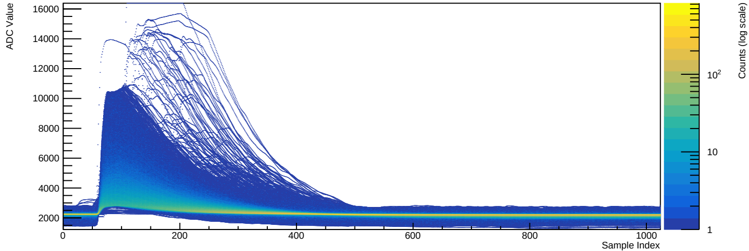
Run 039503 - Channel 2080 (n=28528 waveforms)
