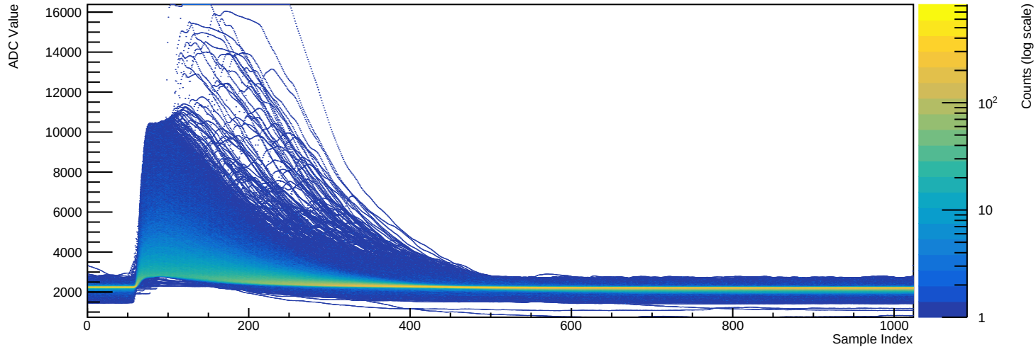
Run 039504 - Channel 2080 (n=29678 waveforms)
