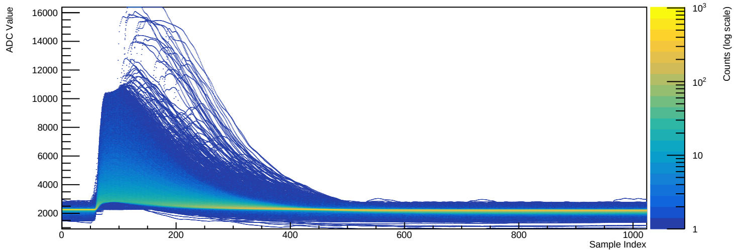
Run 039508 - Channel 2080 (n=35501 waveforms)
