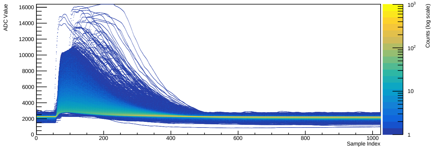
Run 039510 - Channel 2080 (n=38593 waveforms)
