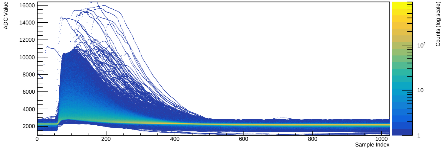
Run 039512 - Channel 2080 (n=35509 waveforms)
