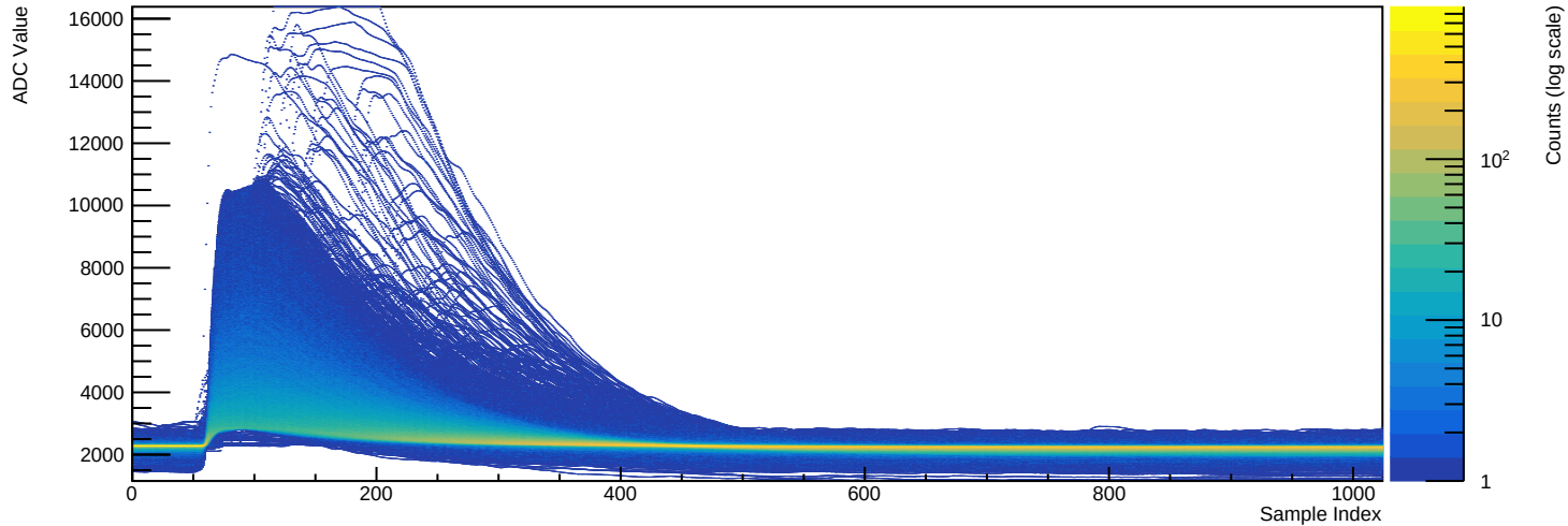
Run 039514 - Channel 2080 (n=33915 waveforms)
