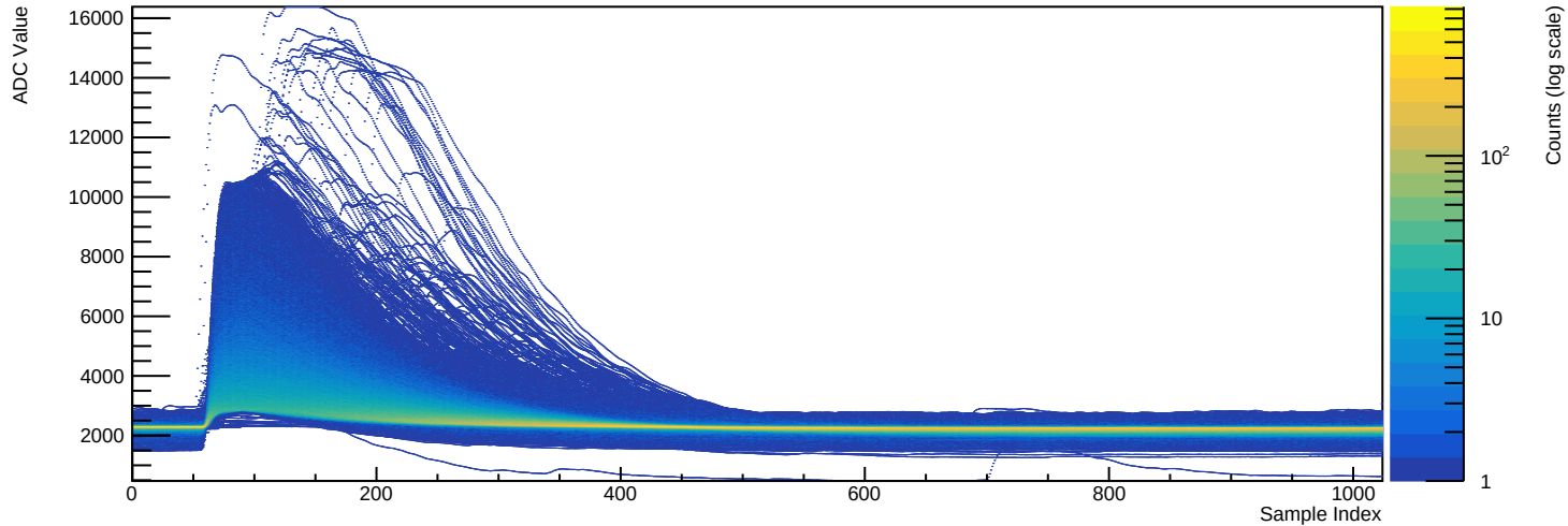
Run 039517 - Channel 2080 (n=30921 waveforms)
