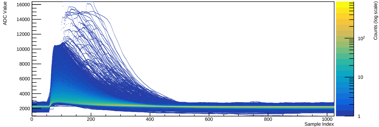
Run 039518 - Channel 2080 (n=30238 waveforms)
