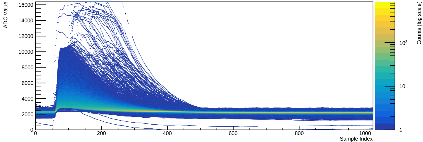
Run 039519 - Channel 2080 (n=29163 waveforms)
