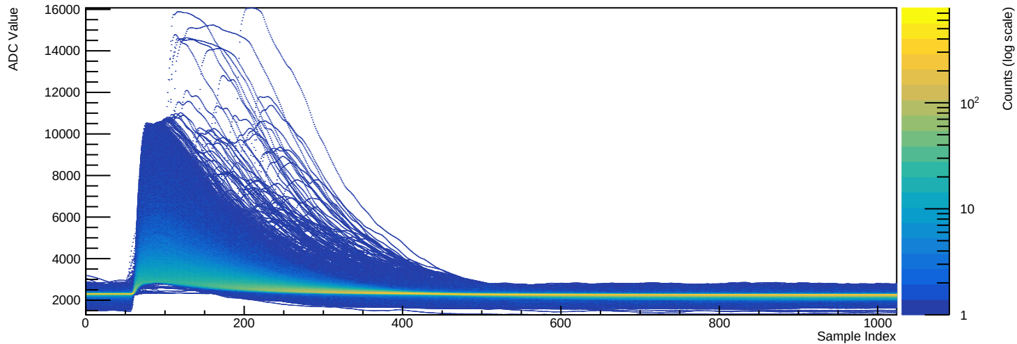
Run 039525 - Channel 2080 (n=25913 waveforms)
