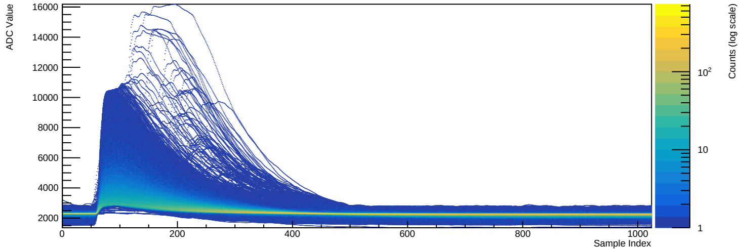
Run 039528 - Channel 2080 (n=24691 waveforms)
