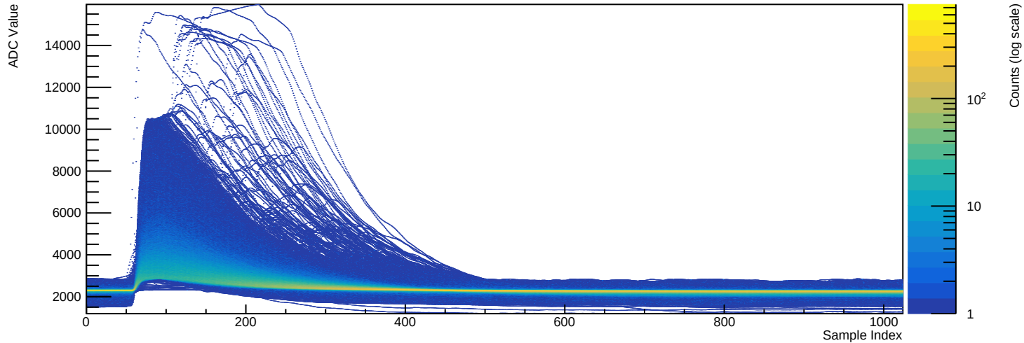
Run 039529 - Channel 2080 (n=24240 waveforms)
