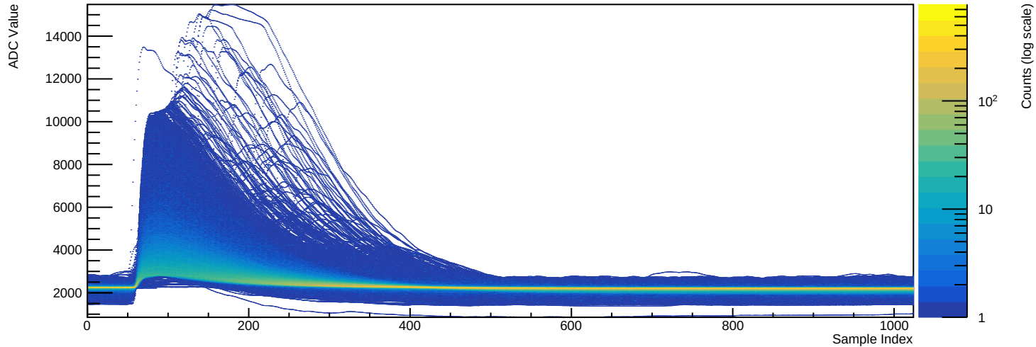
Run 039501 - Channel 2081 (n=25227 waveforms)
