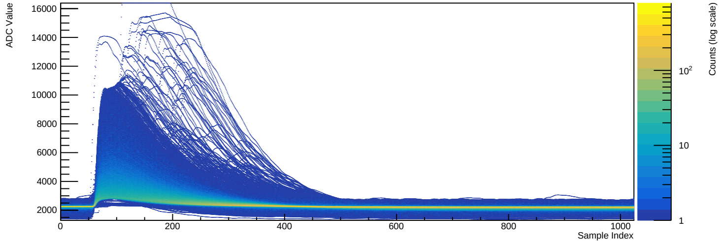
Run 039503 - Channel 2081 (n=27934 waveforms)
