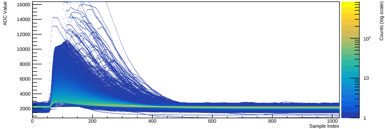
Run 039504 - Channel 2081 (n=29224 waveforms)
