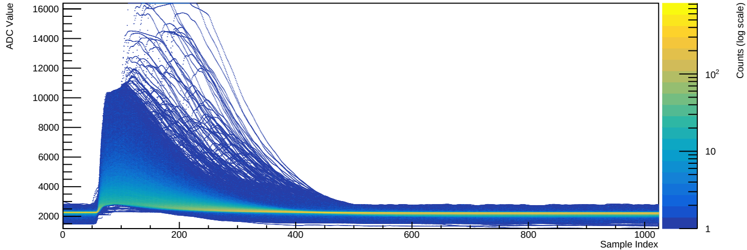
Run 039506 - Channel 2081 (n=30936 waveforms)
