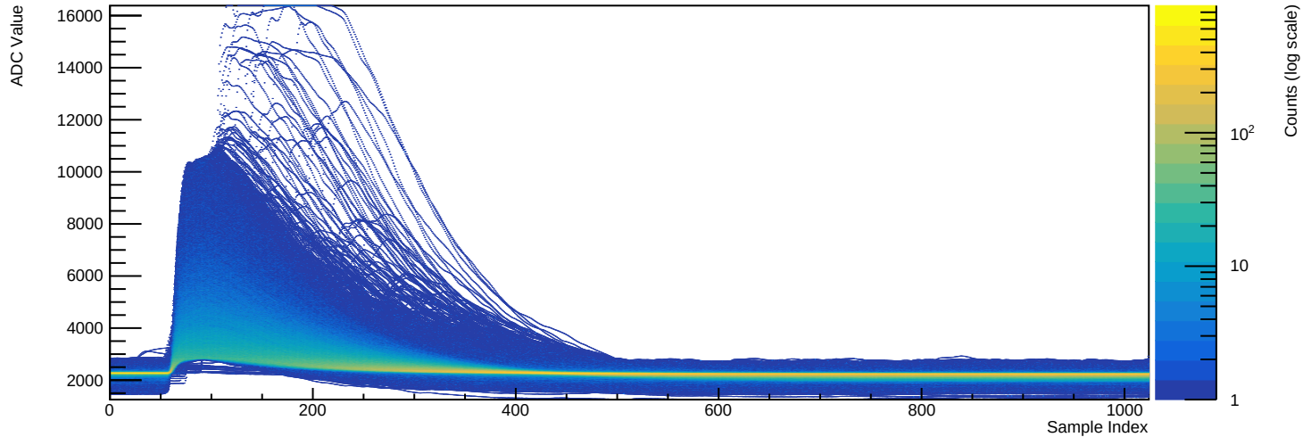
Run 039507 - Channel 2081 (n=33118 waveforms)
