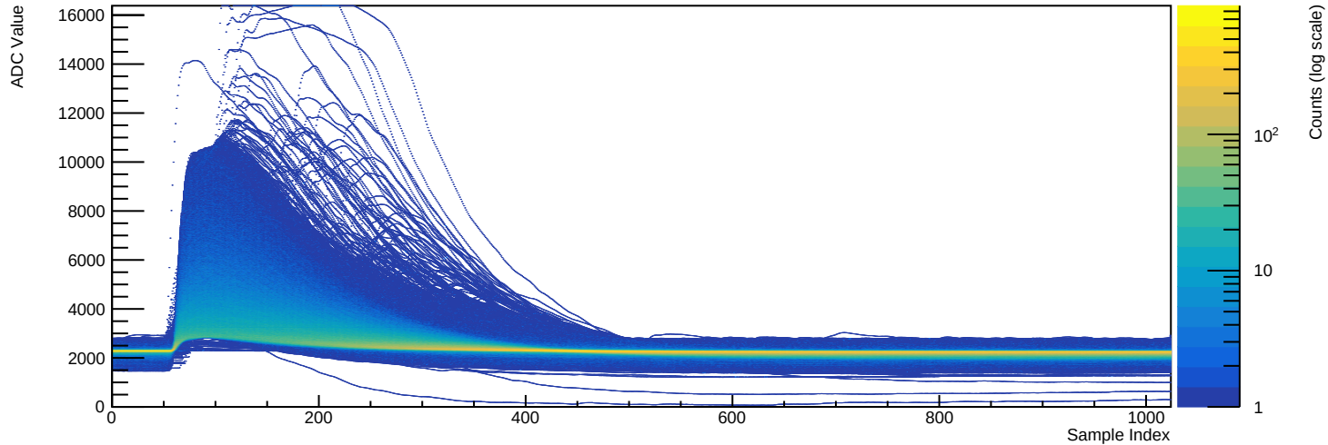
Run 039511 - Channel 2081 (n=37298 waveforms)
