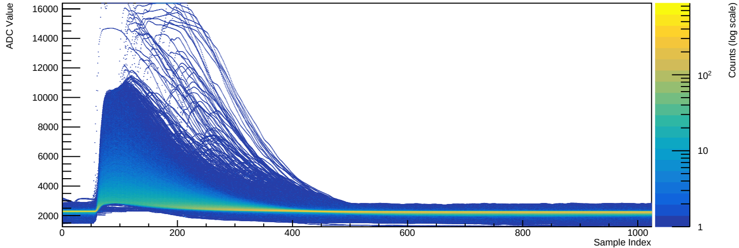
Run 039514 - Channel 2081 (n=33359 waveforms)
