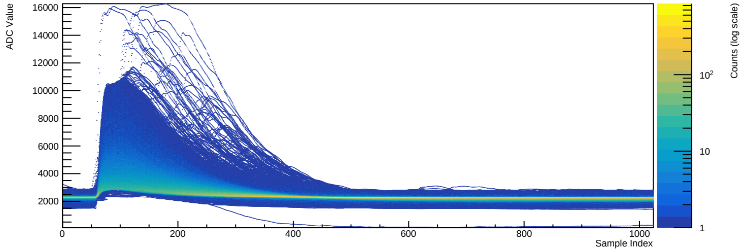
Run 039515 - Channel 2081 (n=31555 waveforms)
