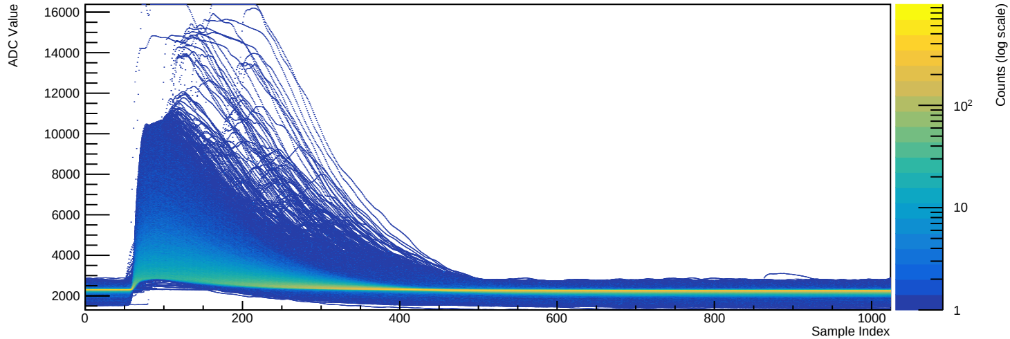
Run 039516 - Channel 2081 (n=30535 waveforms)
